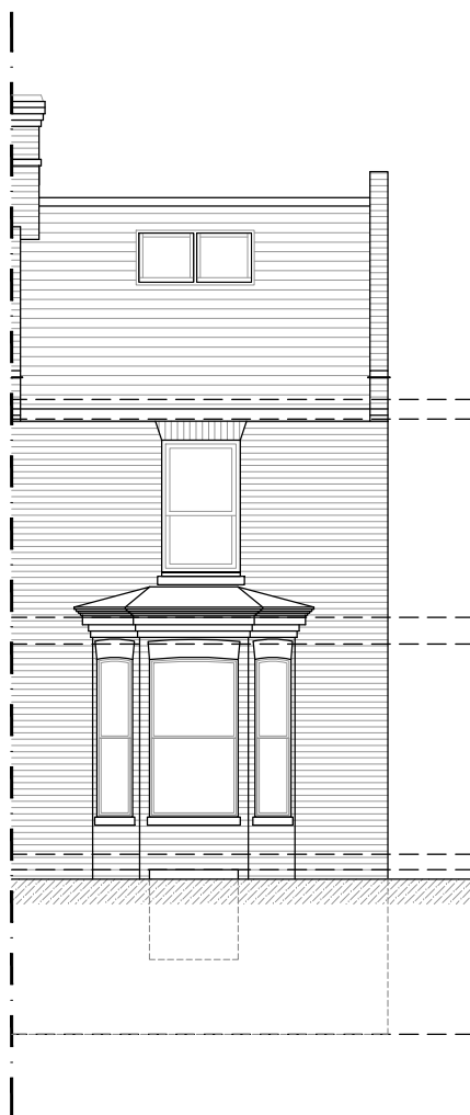
Front (North-West Facing) Elevation 1:100
